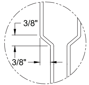
Square profile
