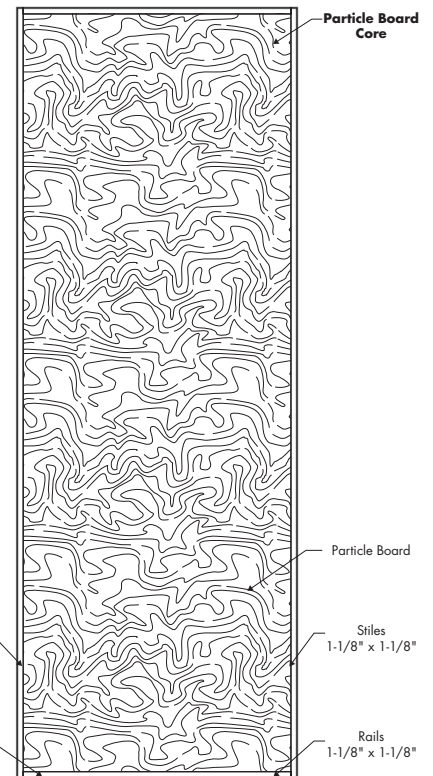
SOLID CORE CONSTRUCTIONS
