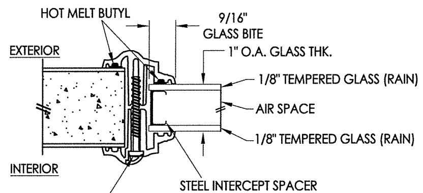
G2 GLAZING DETAIL ODL LITE FRAME (EVOLVE)
