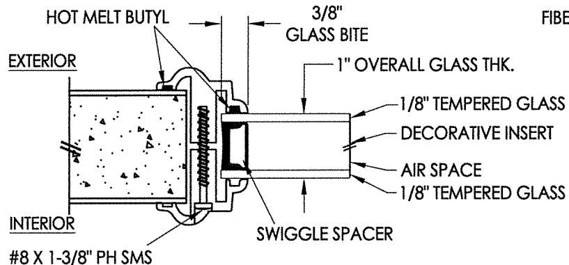
G1 GLAZING DETAIL TKI PRODUCTS LITE FRAME
