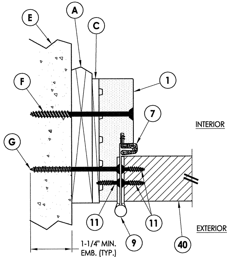
1 HORIZONTAL CROSS SECTION Shown w/ 1X Buck Outswing shown (Inswing similar)
