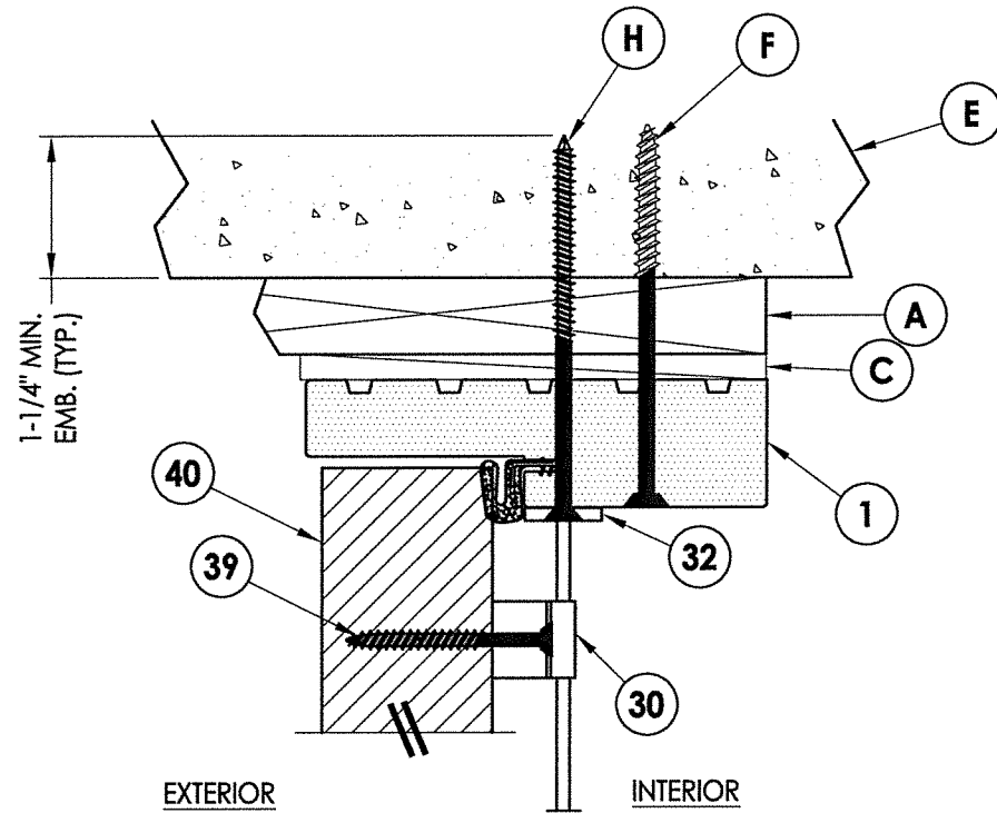
2 VERTICAL CROSS SECTION Shown w/ 1X Buck Outswing shown
