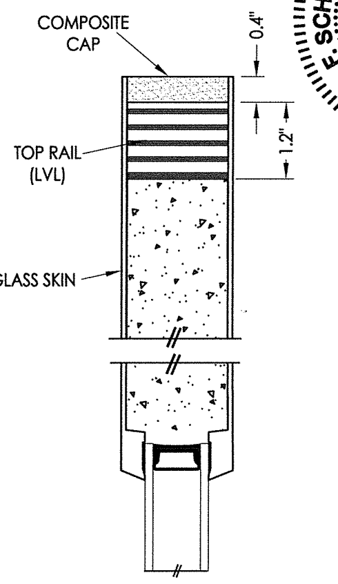
2 VERTICAL CROSS SECTION
