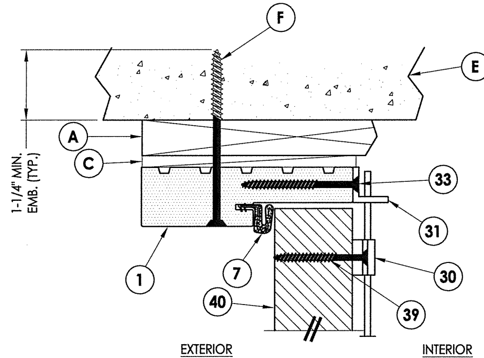
3 VERTICAL CROSS SECTION Shown w/ 1X Buck Inswing shown
